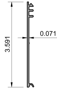
4 FLUSH ADAPTOR SPA10007 6063-T5
