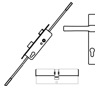
16 DOOR LOCK & HANDLE & CYLINDER DS1297
