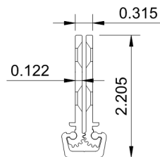
15 CONTINUOUS HINGE YHG004
