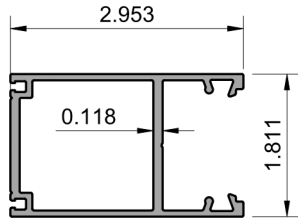
3 DOOR STILE SPA10014 6063-T5
