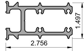
10 CONNECTING ADAPTOR YYS046 6063-T5
